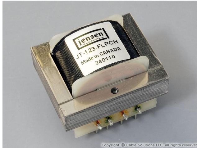
Figure 3.X: “Jensen Transformers JT-123-FLPCH Line Output Transformer, PCB Mount” (reference cs1.net )
