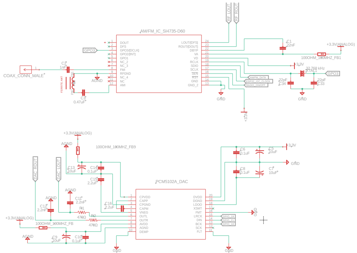
Figure 6.X: Digital-to-Analog Converter and AM/FM IC
