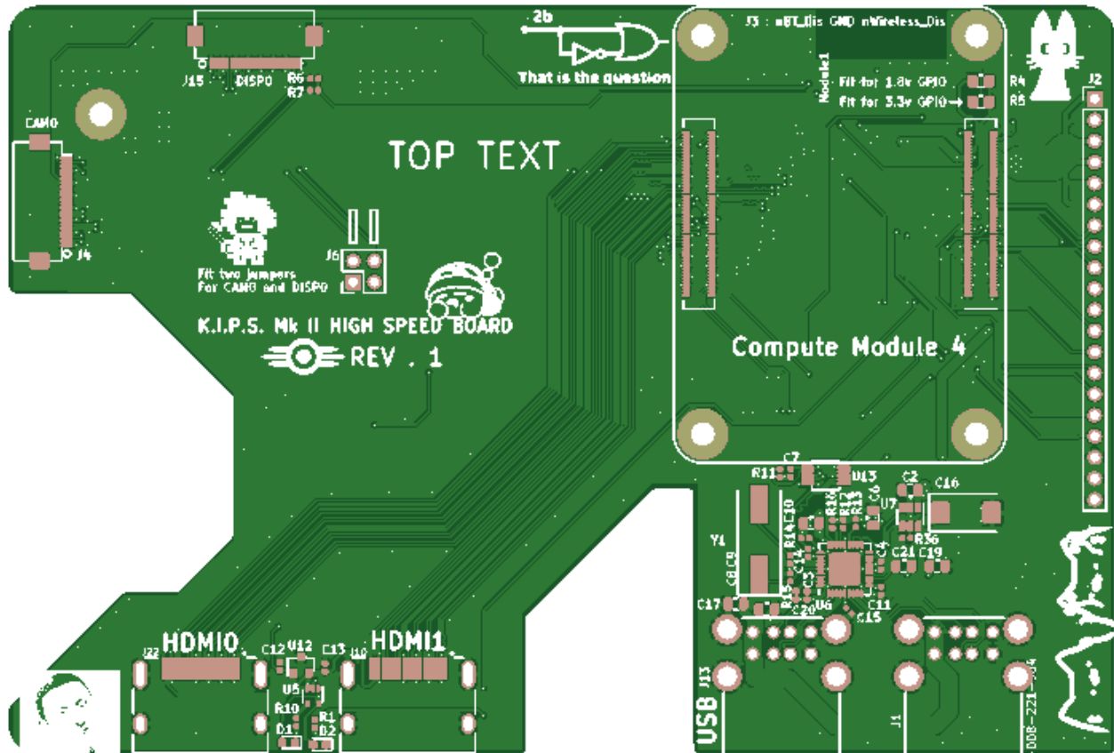
Figure 8.x: 2D High speed Board Layout 8.3 Regulator PCB
