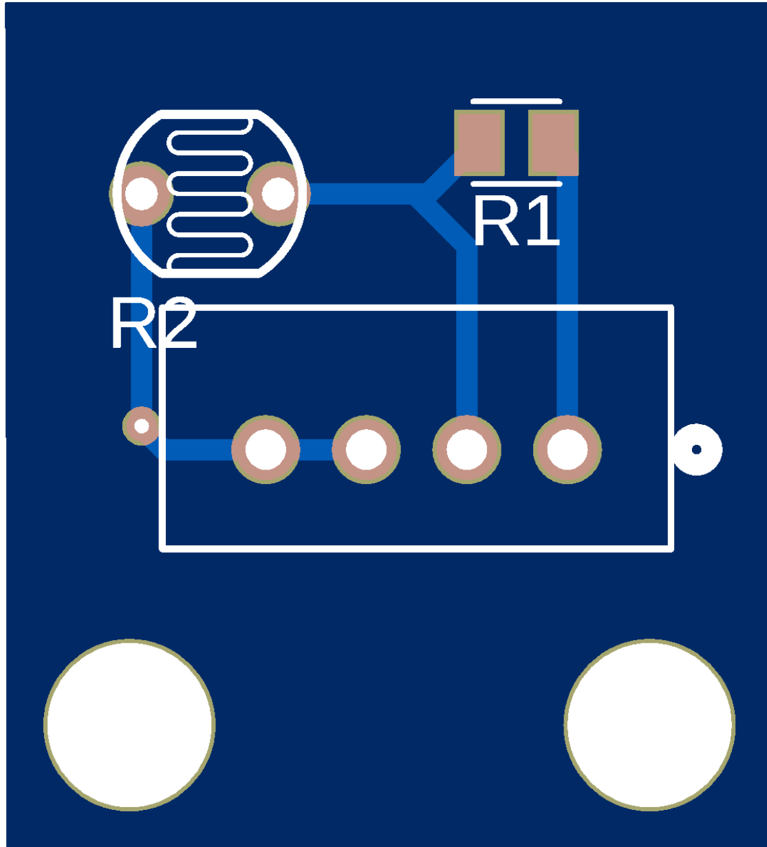
Figure 8.x: Photoresistor sensor Board Layout
