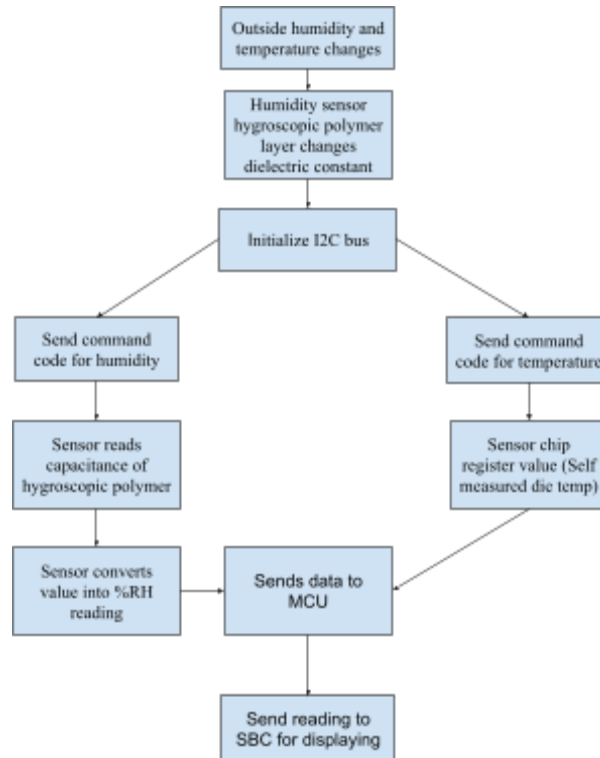
Figure 7.X Temperature and Humidity Sensor Polling Algorithm by Authors
